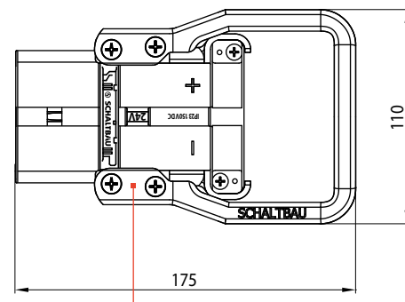
Screw-on handle LV160/320-H-bk/S, black [●] LV160/320-H-rd/S, red [●]
