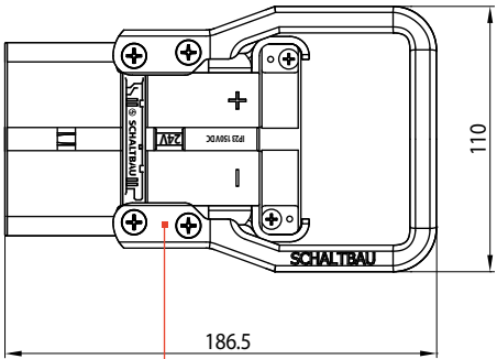
Screw-on handle LV160/320-H-bk/S, black [●] LV160/320-H-rd/S, red [●]
