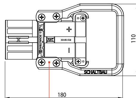
Screw-on handle LV160/320-H-bk/S, black [●] LV160/320-H-rd/S, red [●]
