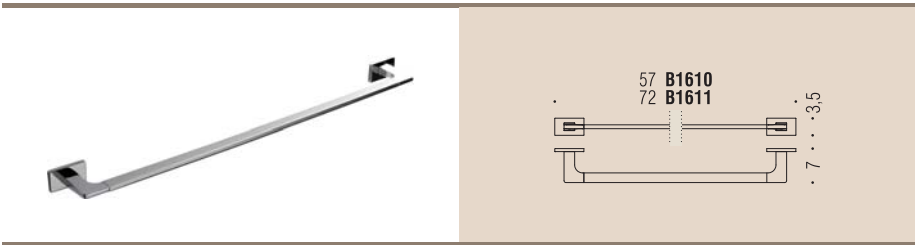
B1610 - B1611 Porta salvietta Towel holder ● ● ●
