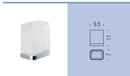
W4202 Porta bicchiere Glass holder
