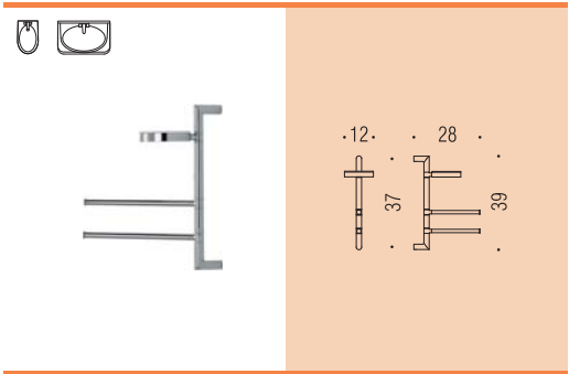
B9824 Colonna con porta sapone e 2 porta salvietta Wall column with soap holder and 2 towel holders
