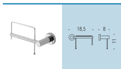
W4908DX - W4908SX Porta rotolo Paper holder
