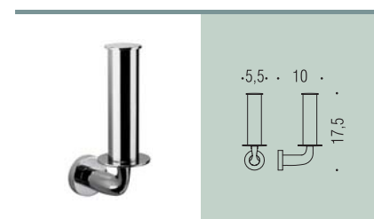
B2790 Porta rotolo Paper holder
