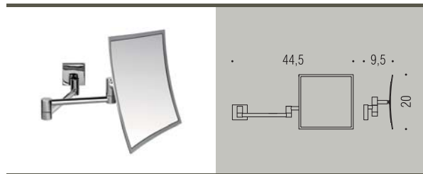
B9754 Specchio ingranditore (3x) a muro Wall magnifying mirror (3 times)
