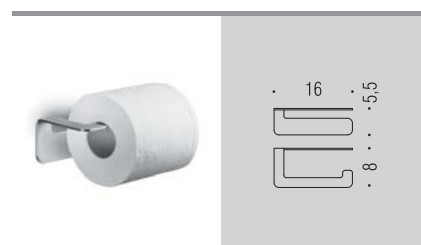
B7008 - B7008V Porta rotolo Paper holder
