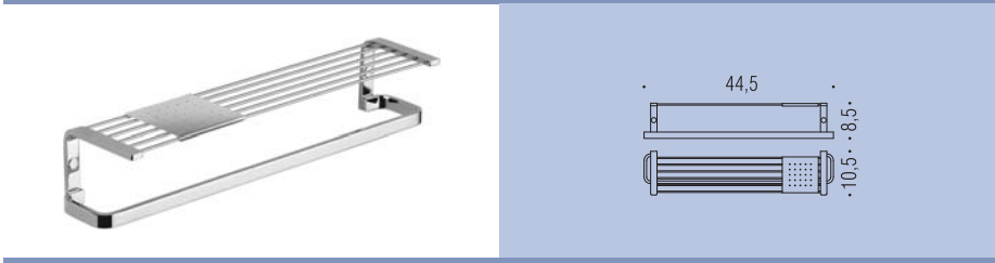
W4277 Mensola con porta salvietta e ripiano in inox Shelf with towel holder and stainless steel tray
