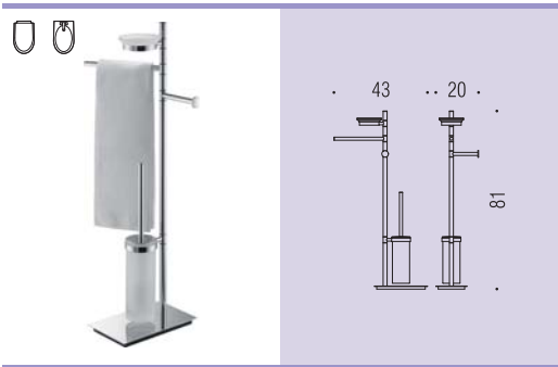
B9903 Piantana con porta salvietta, porta sapone, porta rotolo e porta scopino sospeso in vetro acidato Floor standing column with towel holder, soap holder, paper holder and suspended acid glass brush holder
