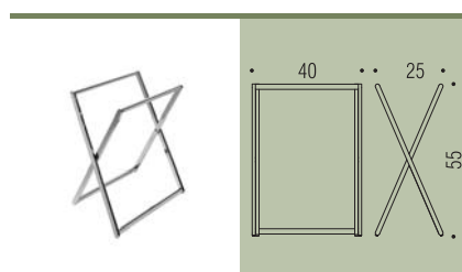
B9736 “Cavalletto” porta salviette H.55 Rack H=55cm
