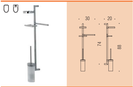
B9822 Colonna con porta sapone, porta salvietta, porta rotolo, porta scopino in vetro acidato Wall column with soap holder, towel holder, paper holder and acid glass brush holder
