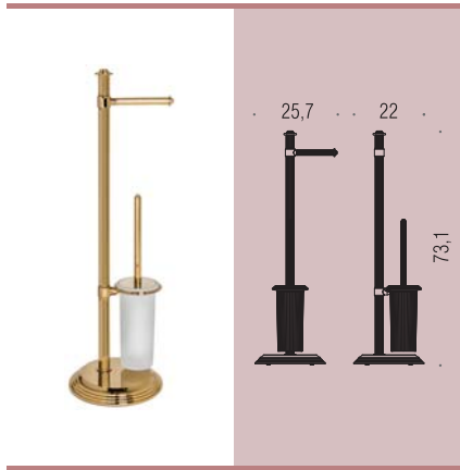
B3318 Piantana con porta rotolo e porta scopino Standing column with paper holder and brush holder
