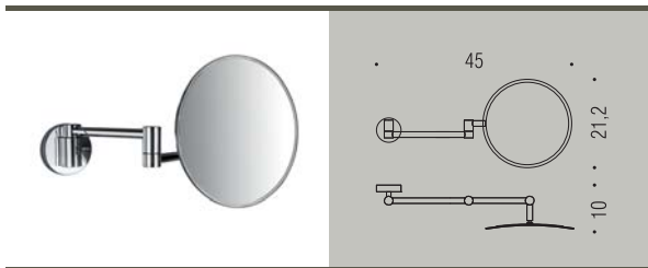
B9759 Specchio ingranditore (3,3x) a muro Wall magnifying mirror (3,3 times)
