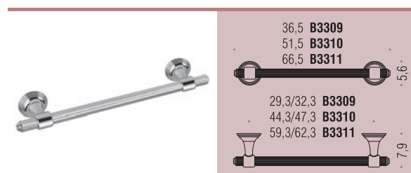
B3309 - B3310 - B3311 Porta salvietta Towel holder
