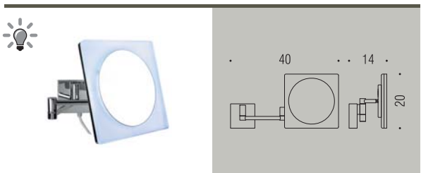
B9756 Specchio ingranditore (3x) a muro con luce a LED incorporata Wall magnifying mirror (3 times) complete with LED built-in light
