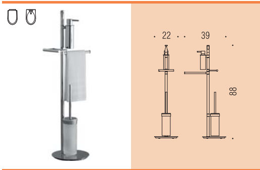
B9849 Piantana con spandisapone (L 0,15), porta salvietta, porta rotolo e porta scopino sospeso in vetro acidato Floor standing column with soap dispenser, towel holder, paper holder and suspended acid glass brush holder
