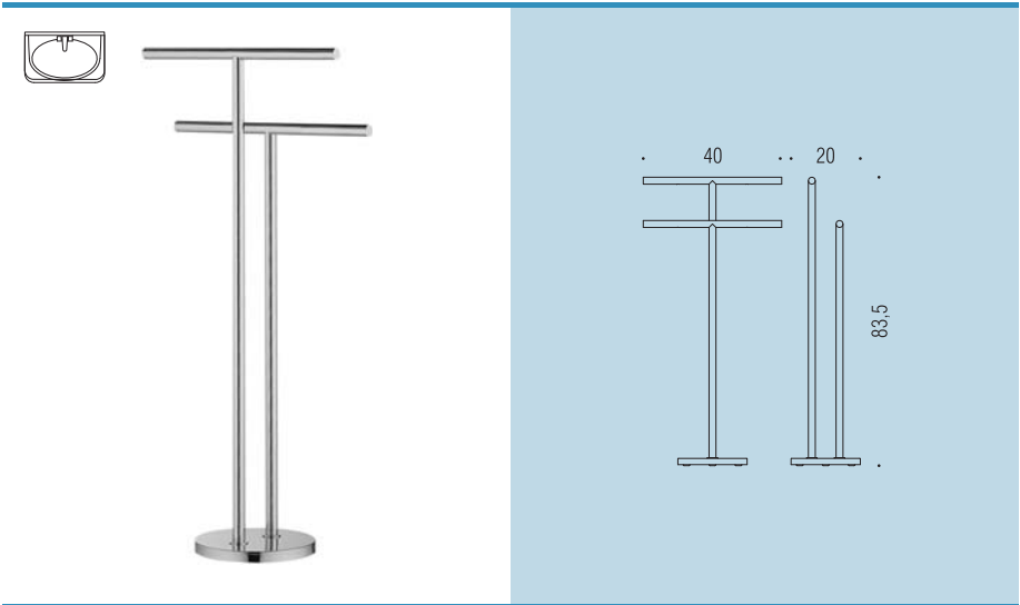
W4938 Piantana con due porta salvietta Standing column equipped with two towel holders
