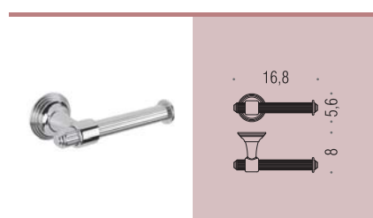
B3308 Porta rotolo Paper holder
