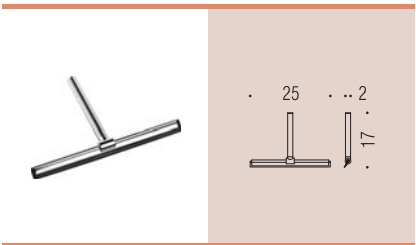
B9636 Tergivetro “AQUACLEAN” “AQUACLEAN” Glass wiper
