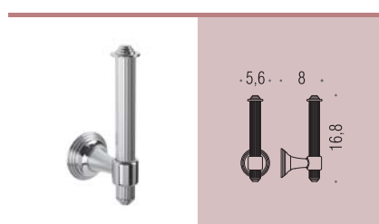
B3390 Porta rotolo Paper holder
