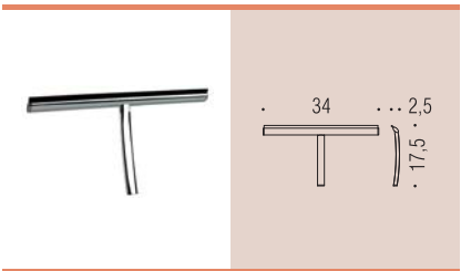
B9643 Tergivetro Glass wiper
