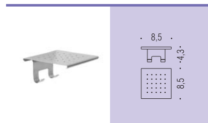
B9644 Mensola con gancio per tergivetro (B9636-B9643) Shelf with hook for glass wiper
