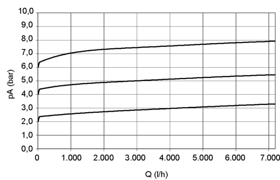
Characteristic curve DN 32
