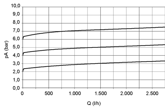
Characteristic curve DN 25
