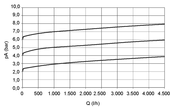
Characteristic curve DN 32
