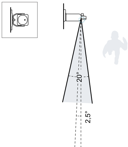
Top view with sensor inclination 0°.
