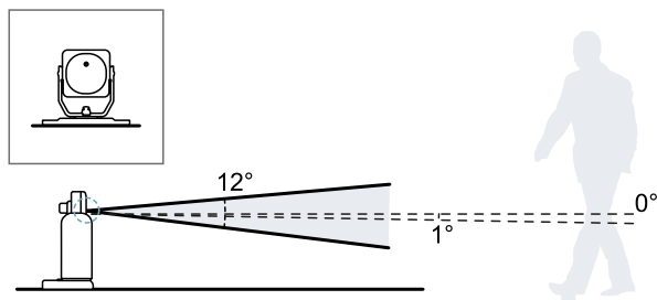
Side view with sensor inclination 0°.
