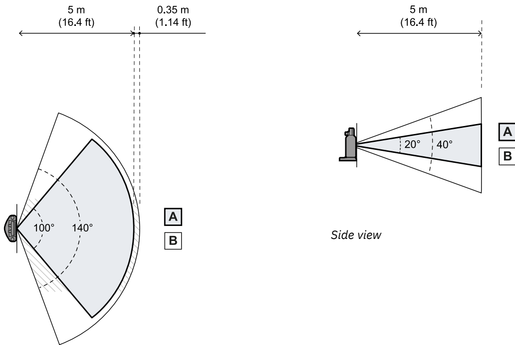
Top view
